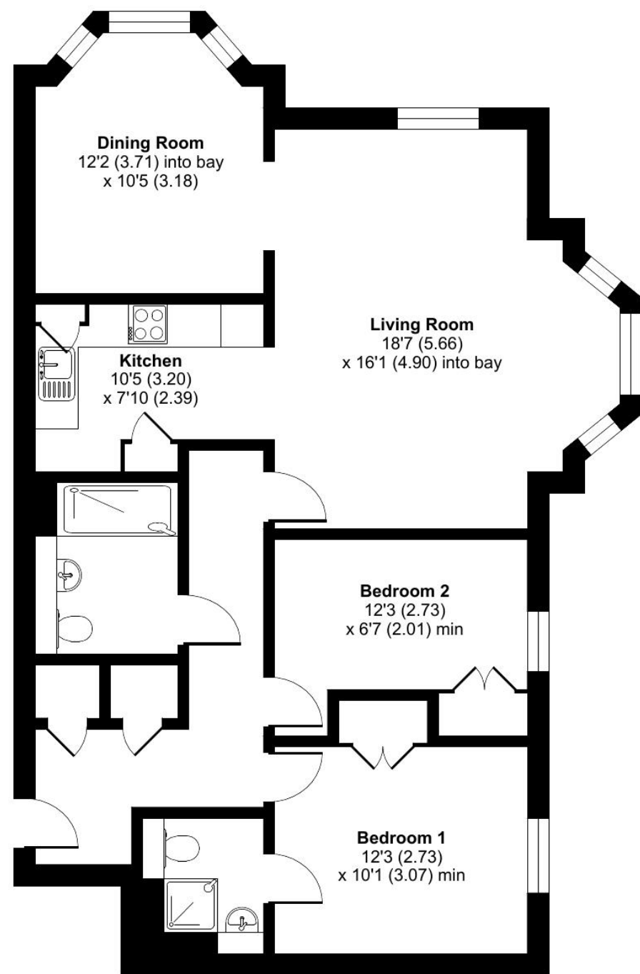
FIRST FLOOR
