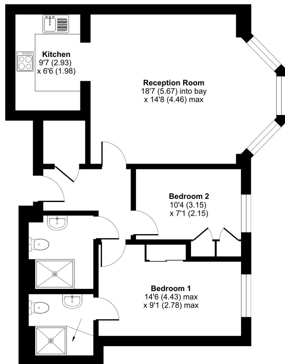
FIRST FLOOR
